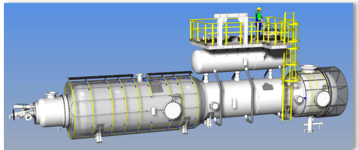
3D Model Thermal Reactor Package
